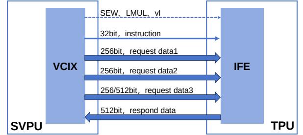
Figure 4: VCIX Interface.
