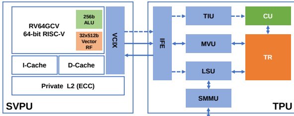
Figure 3: Architecture of RTPU.
