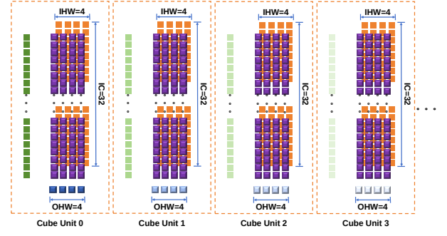
Figure 10: Matrix Multiplication in Cube Units in parallel.
