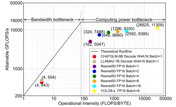
Figure 19: Roofline Model for the OASIS AI Processor.
