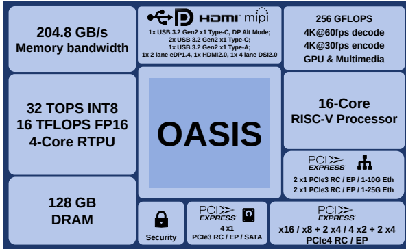
Figure 1: Functional Block of OASIS.
