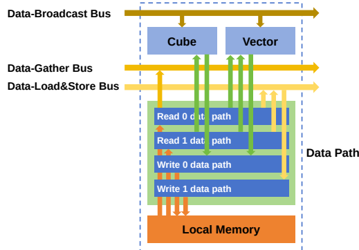
Figure 13: Lane.
