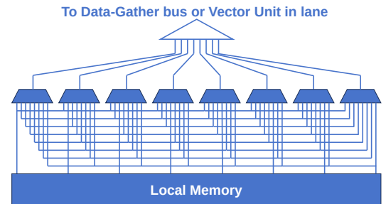
Figure 12: Crossbar.
