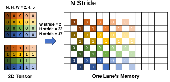
Figure 5: 3D Tensor’s Layout in One STR.
