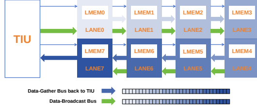
Figure 15: Data-Broadcast Ring Bus.
