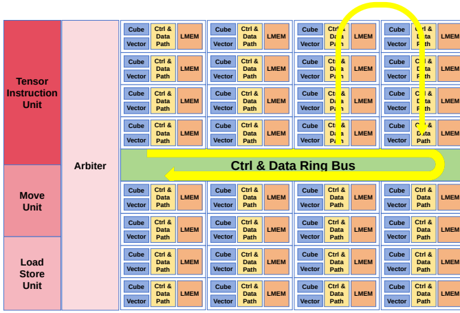
Figure 16: Dual Layer Ring Bus.
