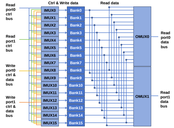
Figure 11: LMEM.
