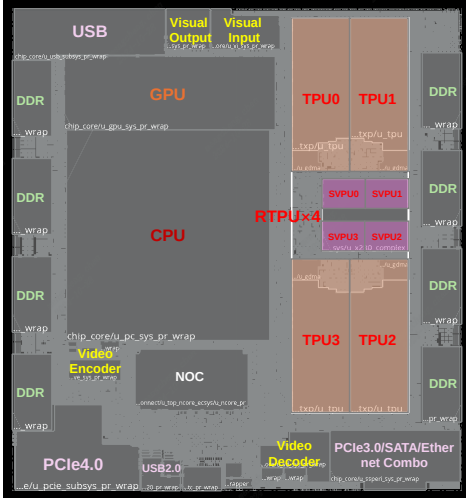
Figure 2: Die photo of OASIS.
