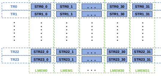
Figure 6: The relationship among TRs, STRs and LMEMs.
