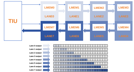
Figure 14: Data-Gather Ring Bus.
